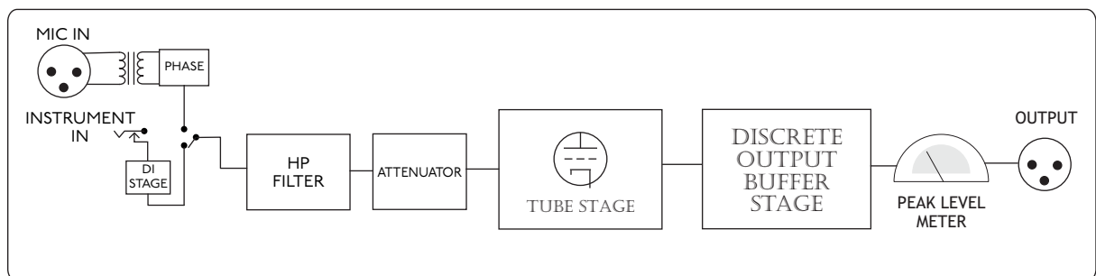
OPERATIONAL BLOCK DIAGRAM (ONE CHANNEL)
